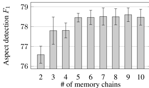
Figure 3: Sensitivity study of model performance to # of memory chains n . Note that we report average performance over 5 runs with standard deviation.
